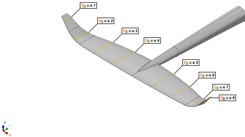
Figure 2 - Definition of Cross Sections
