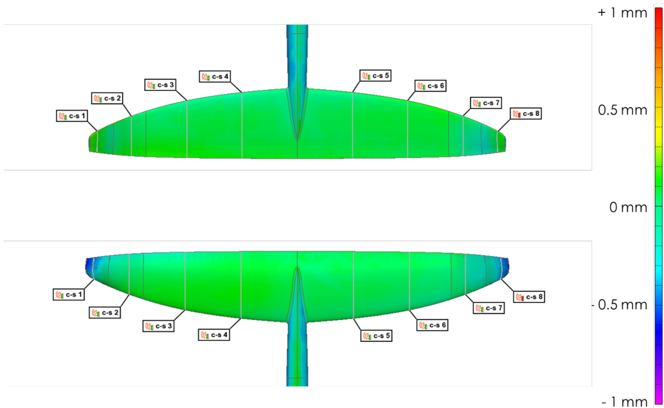
Figure 7 - Colour Map of the Upper (top) and Lower (bottom) surfaces of the Rearwing
