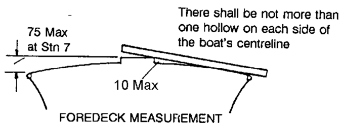
Foredeck Measurement
