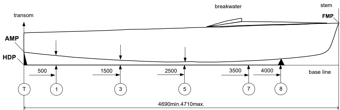
Hull Measurement
